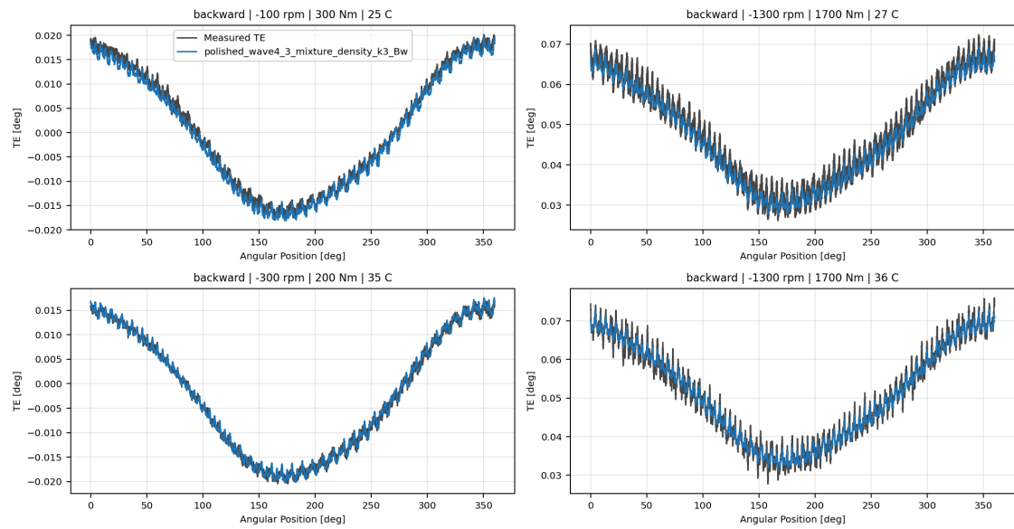
polished_wave4_3_mixture_density_k3_Bw measured-versus-predicted TE collage
