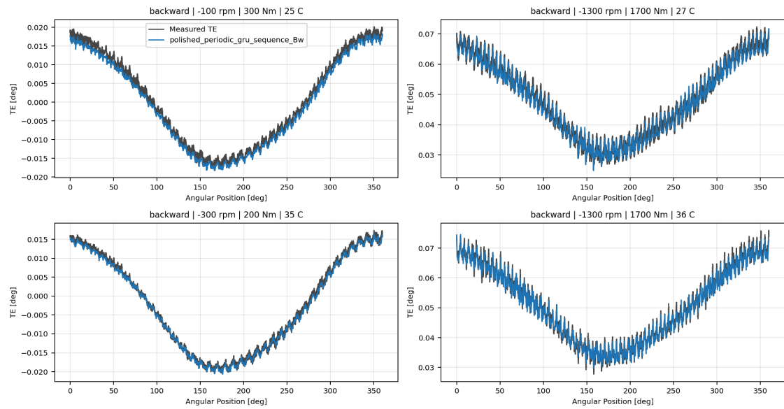
polished_periodic_gru_sequence_Bw measured-versus-predicted TE collage
