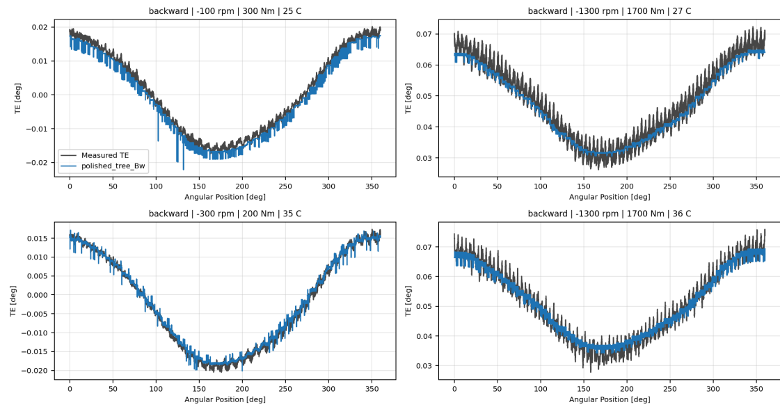
polished_tree_Bw measured-versus-predicted TE collage
