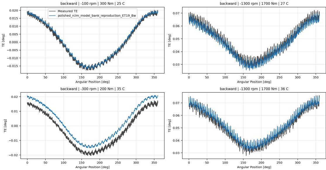
polished_rcim_model_bank_reproduction_ET19_Bw measured-versus-predicted TE collage
