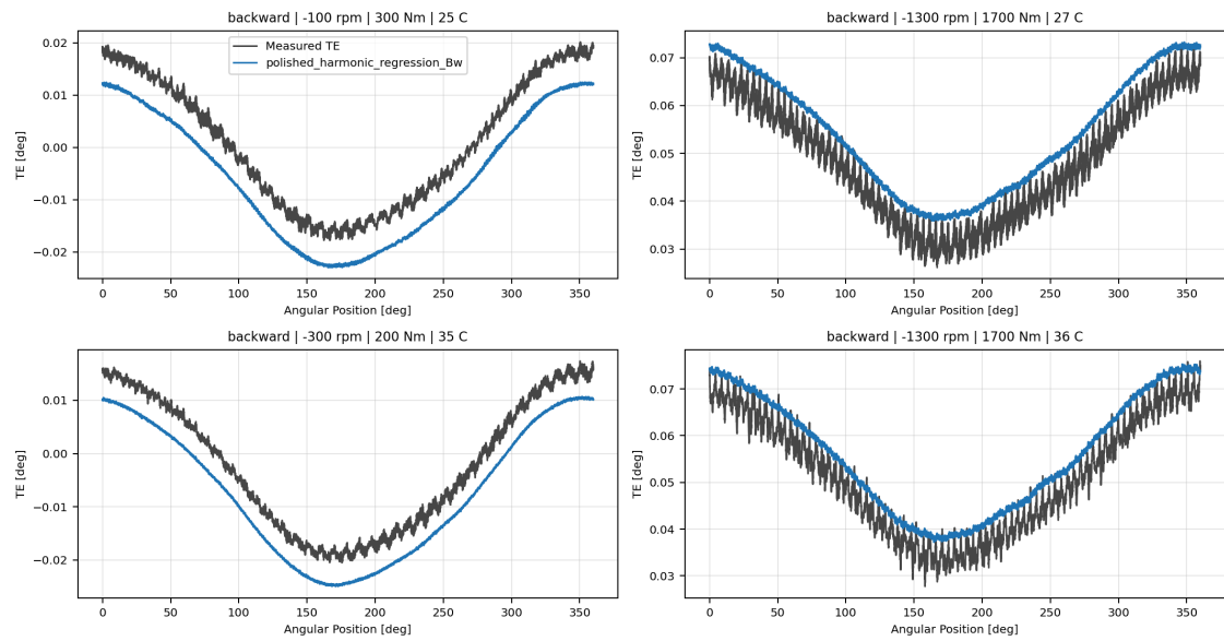
polished_harmonic_regression_Bw measured-versus-predicted TE collage
