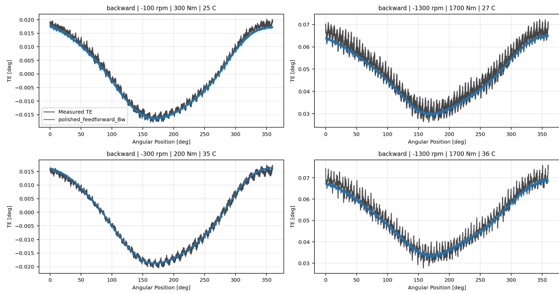
polished_feedforward_Bw measured-versus-predicted TE collage
