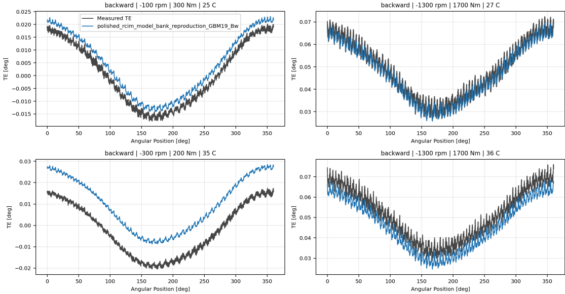
polished_rcim_model_bank_reproduction_GBM19_Bw measured-versus-predicted TE collage
