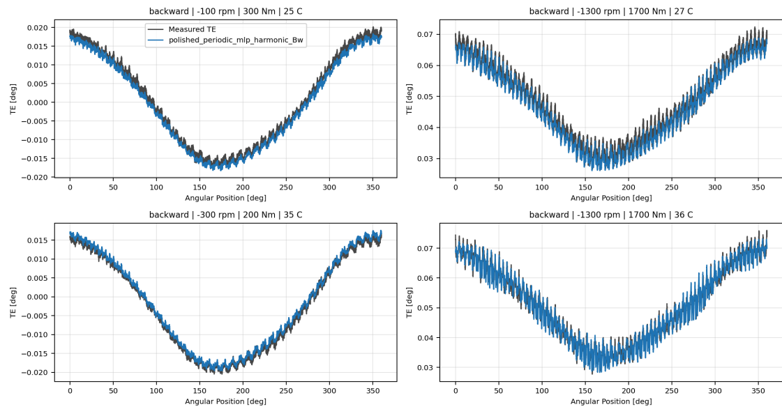
polished_periodic_mlp_harmonic_Bw measured-versus-predicted TE collage
