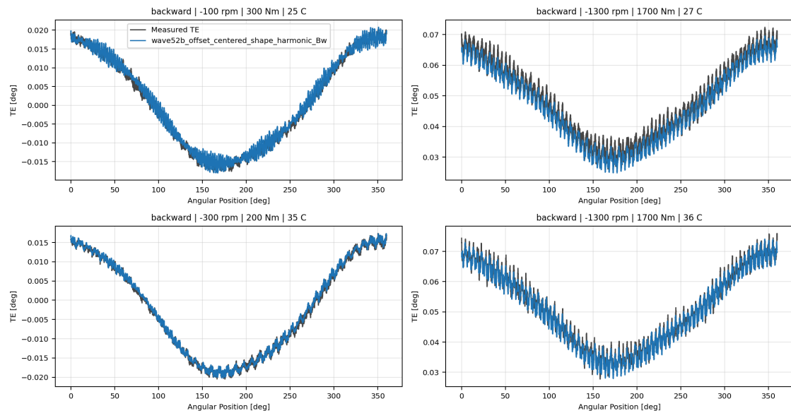
wave52b_offset_centered_shape_harmonic_Bw measured-versus-predicted TE collage
